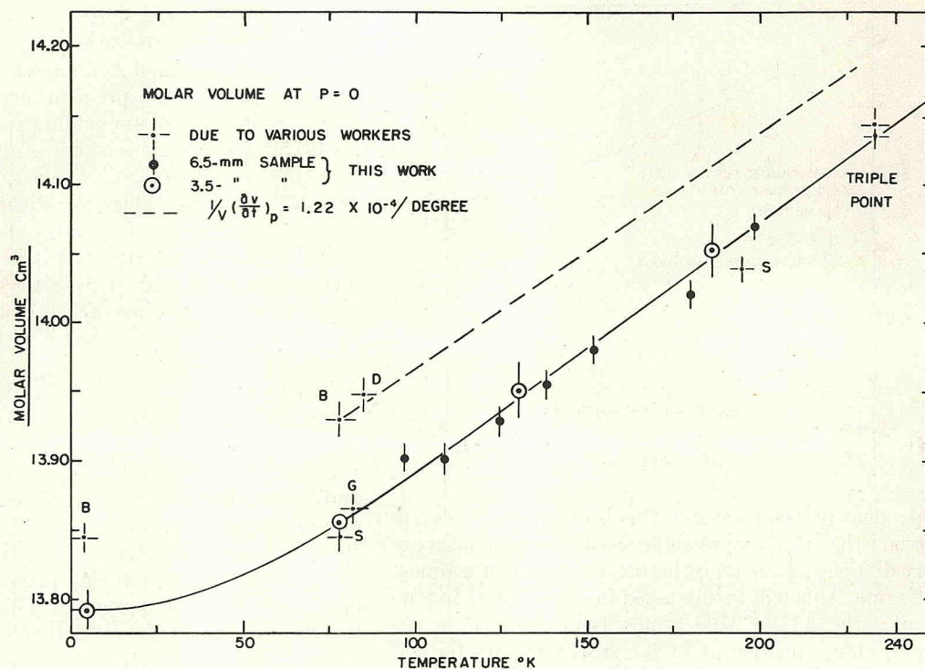
FIG. 7. A summary of the various data for the density of solid \alpha mercury. The letters refer to various workers: G, Grüneisen and Sckell 11 ; S, Sapper and Biltz 11 ; B, Barrett 4 ; D, Dewar. 12 The triple-point densities are as given in the text.
