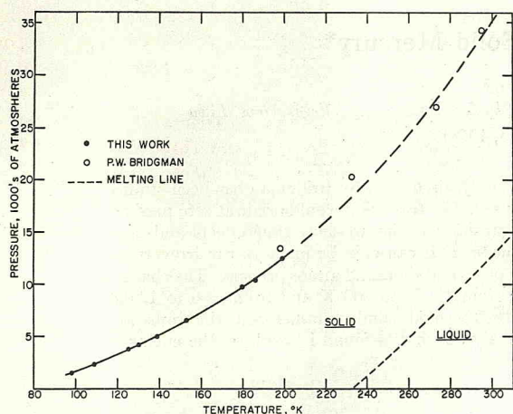
FIG. 1. The phase diagram for solid mercury.
