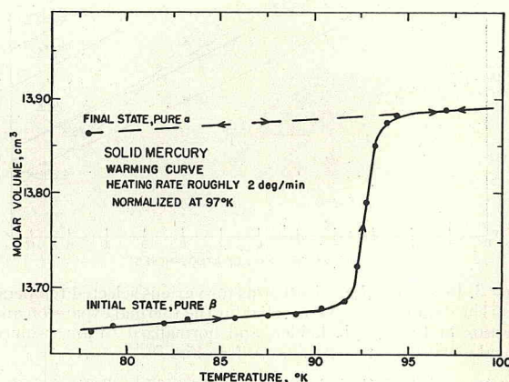
FIG. 4. The warming curve for a sample which was initially in the \beta phase.
